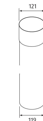
Round downpipe 120 (1000, 2000, 3000 or 4000 long)
