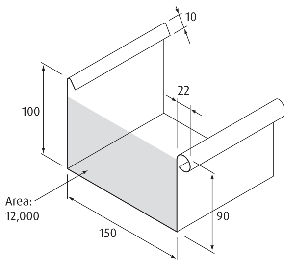
Box gutter (3000 long): Type 400
