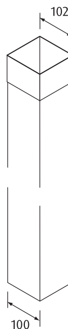
Square downpipes 80 and 100 (1000, 2000 or 3000 long)
