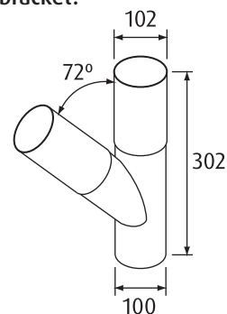
Y branch: 100 dia
