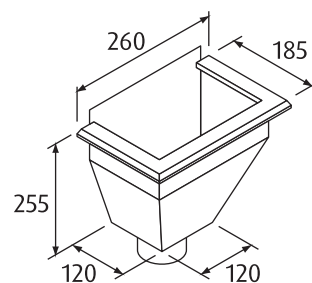
Hopper head: Outlet size 80 or 100
