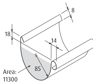
Half round gutter (3000 long): Type 333
