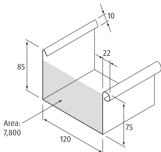
Box gutter (3000 long): Type 333
